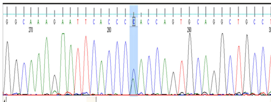
Fig. 2 DNA sequencing of the \beta globin gene showed a mutation in codon 124 CCA \rightarrow CAA, thus identifying the variant as Hb Ty Gard [ \alpha A2 \beta 2 124 (H2) Pro \rightarrow Gln]
