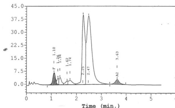
Fig. 1 HPLC chromatographs showing the variant hemoglobin
